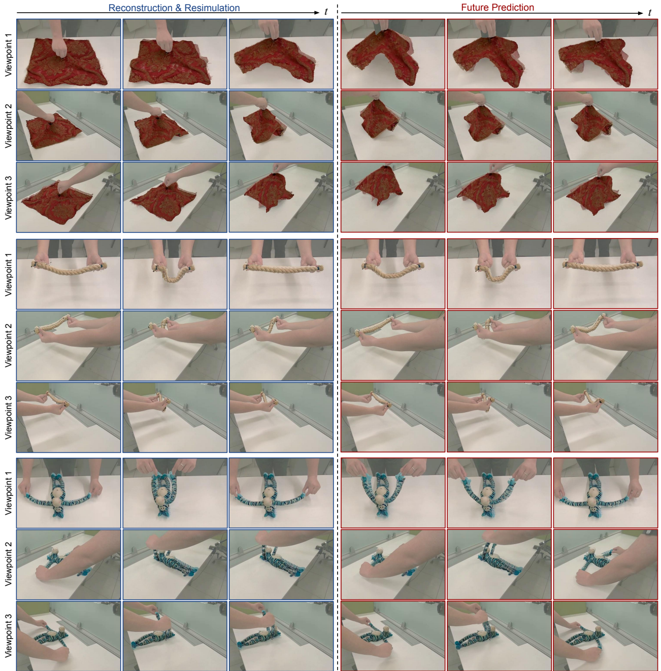
Figure 9. Qualitative Results on Reconstruction & Resimulation and Future Prediction with different viewpoints.
